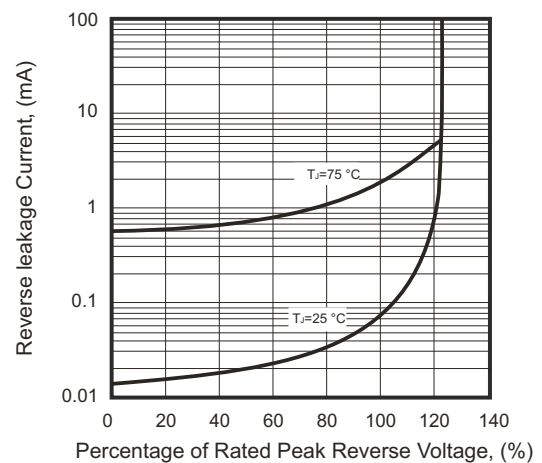
Fig.4 - Typical Revrse Characteristics
