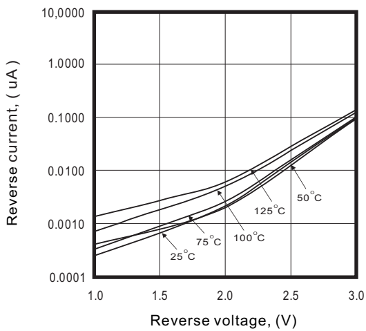
Fig.2 - Reverse characteristic
