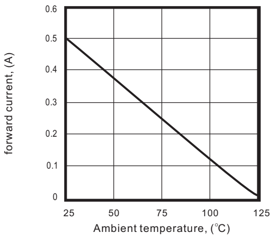
Fig.4 - Power derating
