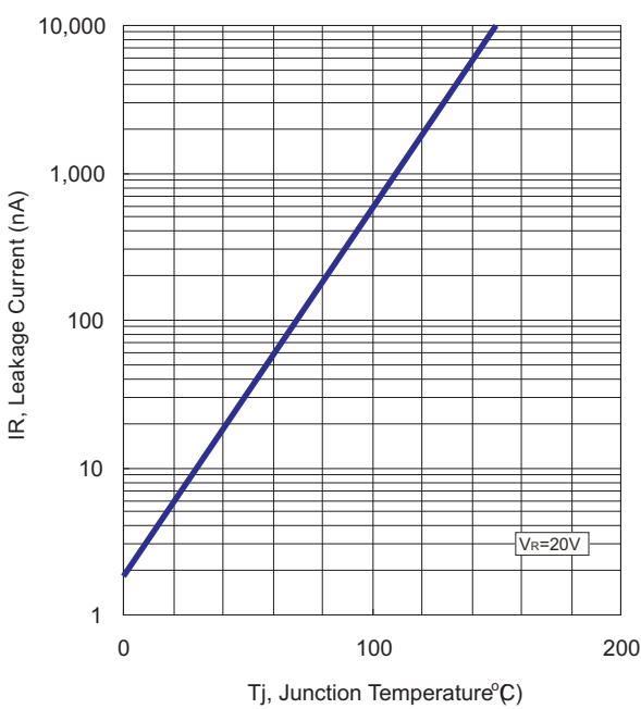
Fig. 2 - Leakage current V.S. Junction Temperature
