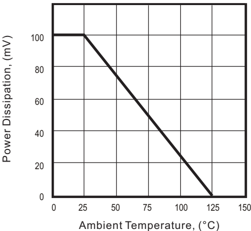
Fig.3 - Derating Curve
