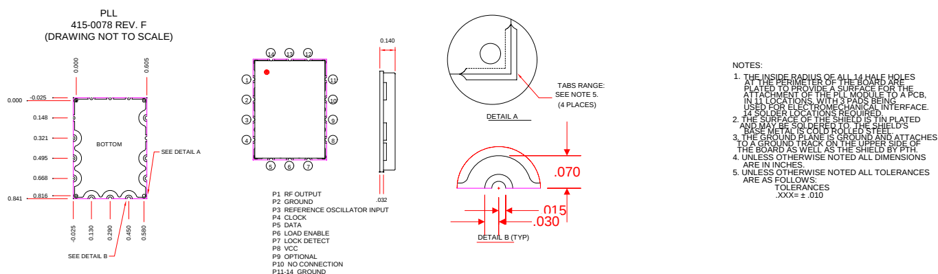
PHYSICAL DIMENSIONS
